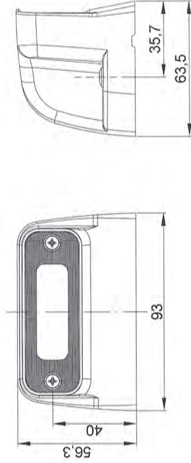
variant FT-263/1 LED registration plate lamp surface mounting
