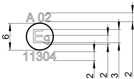
approval dimensions
