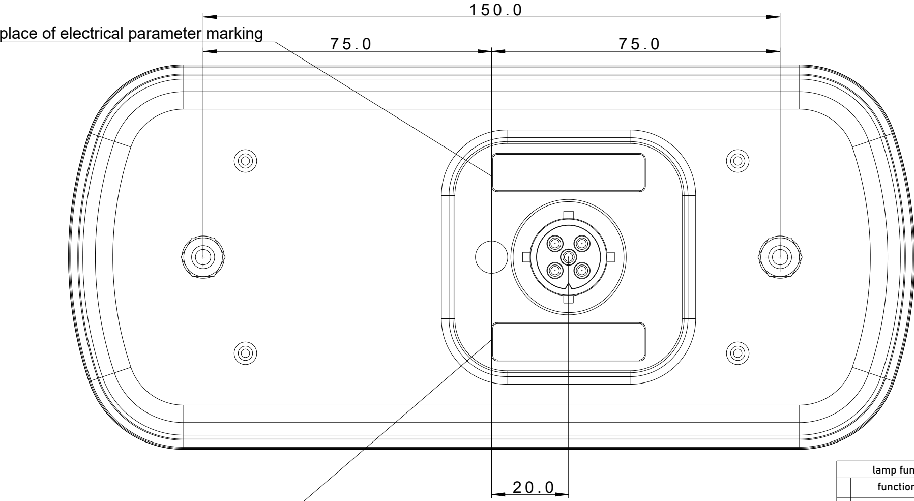
place of electrical parameter marking Left lamp
