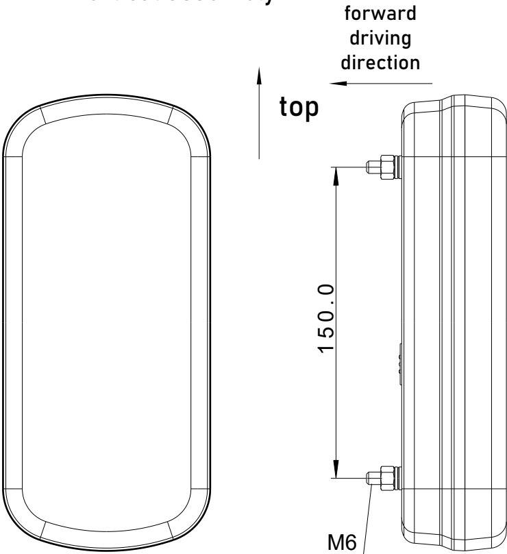
Vertical assembly
