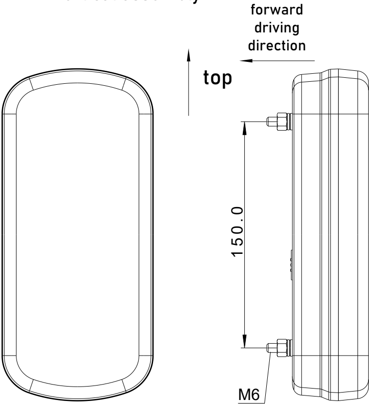
Vertical assembly
